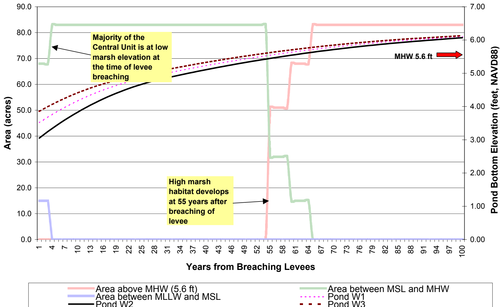
Figure 2-6b. Predicted Tidal Wetland Development in Central Unit
