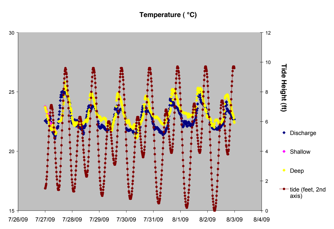
Figure 4.4-9: Pond A14 temperature values at 3 pond locations during 27 July – 2 August
