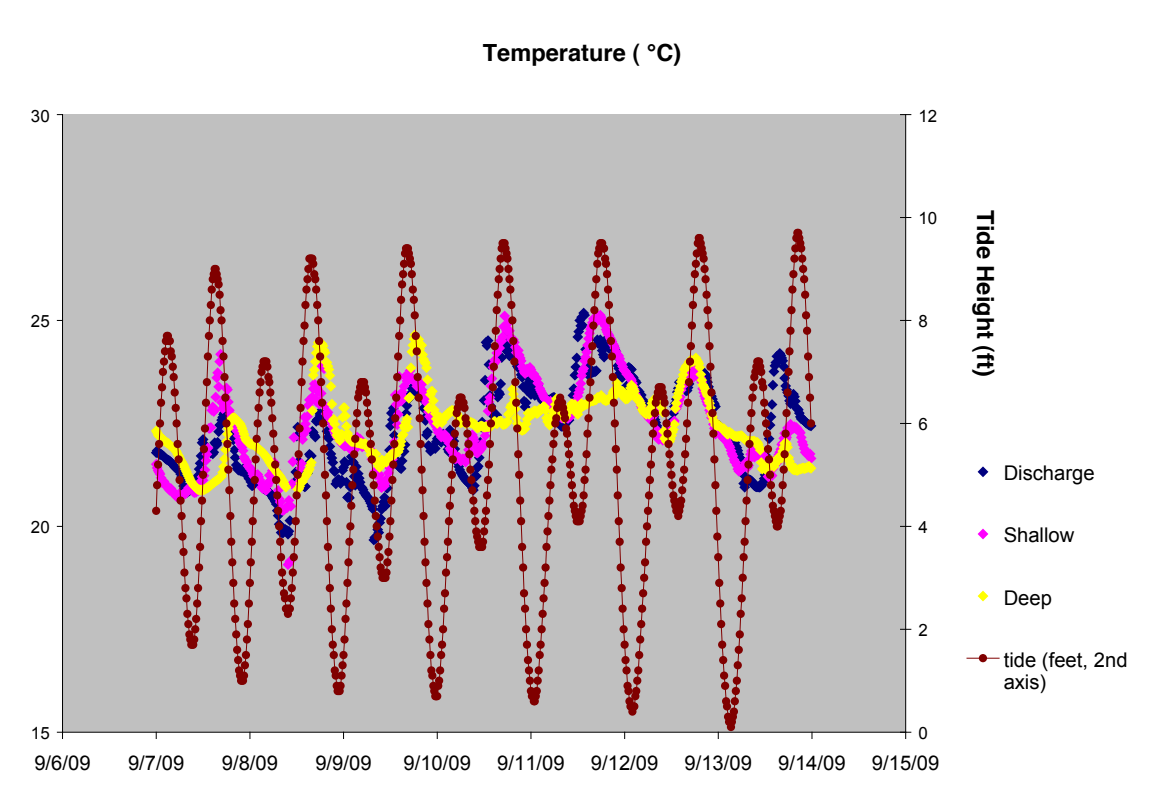
Figure 4.4-15: Pond A14 temperature values at 3 pond locations during 7 September – 13 September
