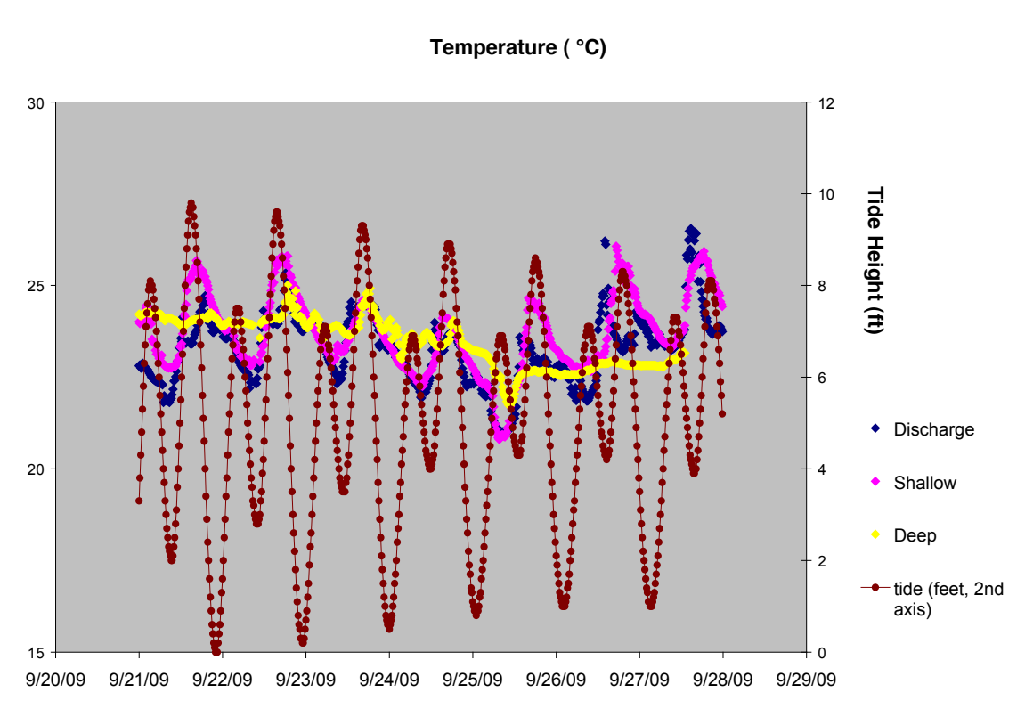
Figure 4.4-17: Pond A14 temperature values at 3 pond locations during 21 September – 27 September
