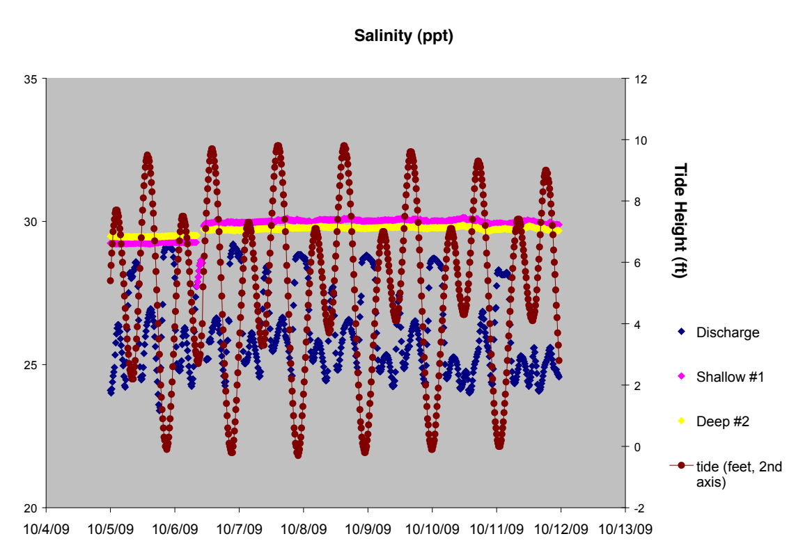
Figure 3.2-19: Pond A3W salinity values at 3 pond locations during 5 October – 11 October
