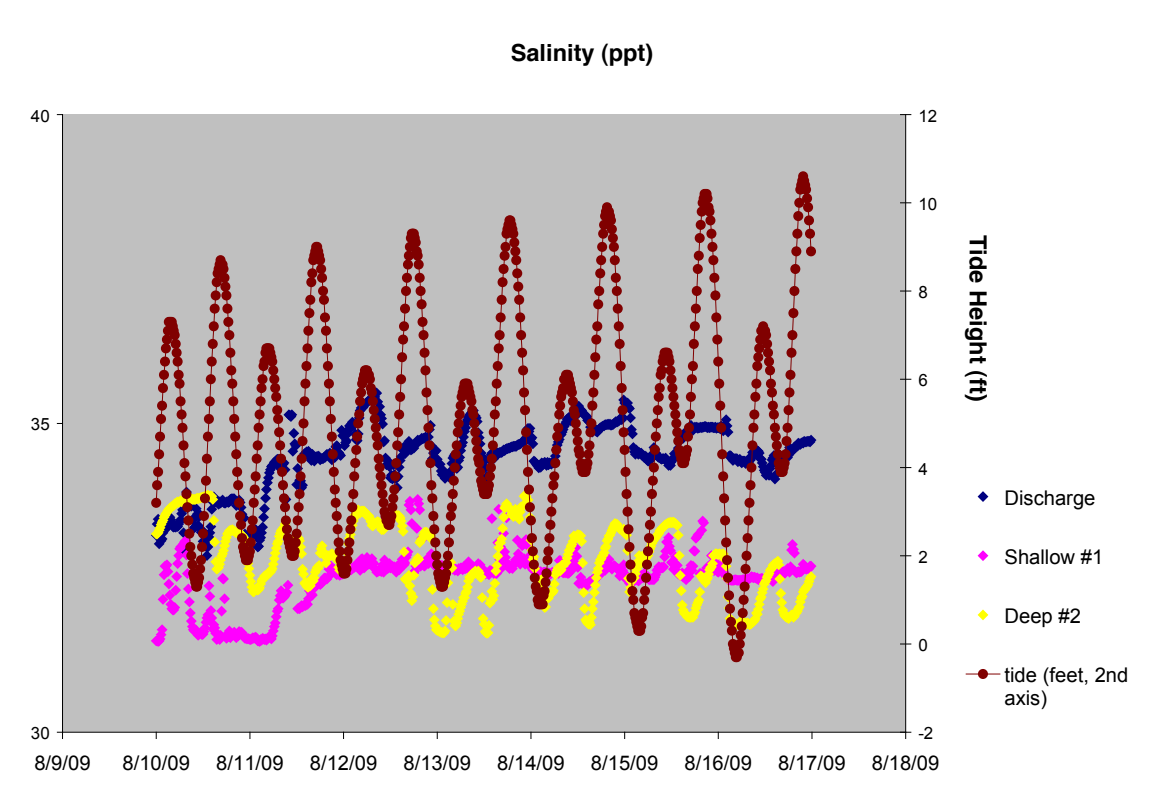
Figure 4.2-11: Pond A14 salinity values at 3 pond locations during 10 August – 16 August
