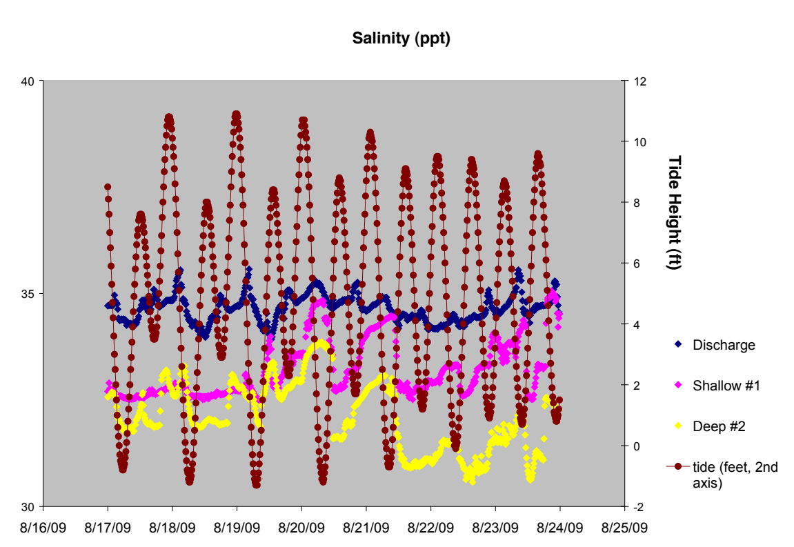
Figure 4.2-12: Pond A14 salinity values at 3 pond locations during 17 August- 23 August
