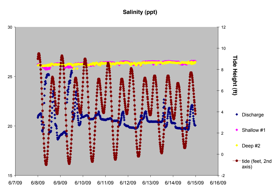
Figure 3.2-2: Pond A3W salinity values at 3 pond locations during 8 June – 14 June
