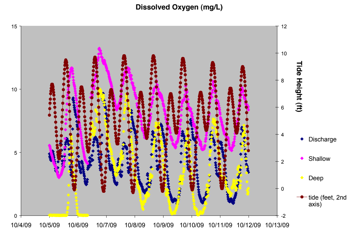
Figure 3.1-20: Pond A3W dissolved oxygen values at 3 pond locations during 5 October – 11 October
