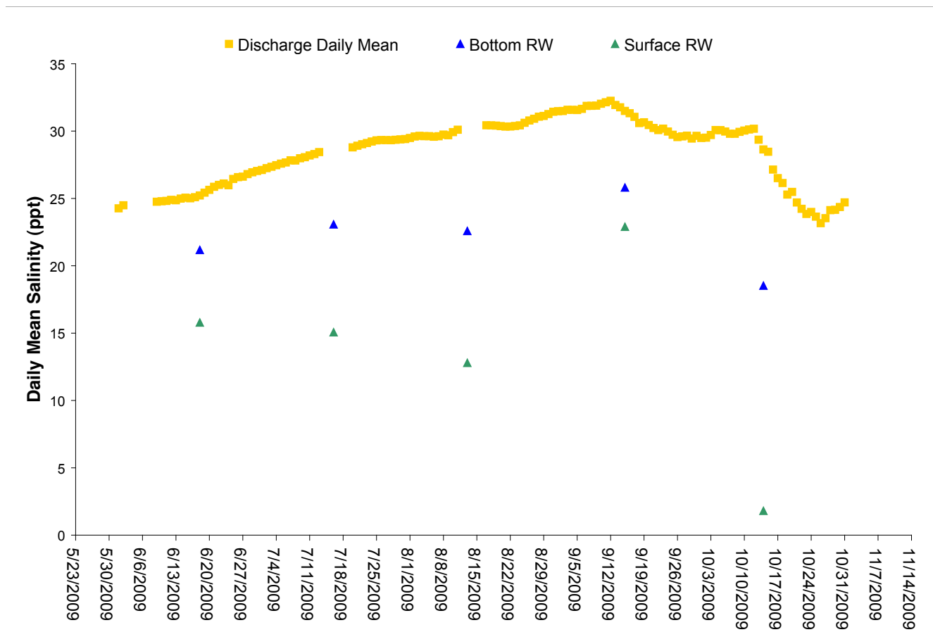
Figure A-15: Salinity of Pond A7 vs. Alviso Slough
