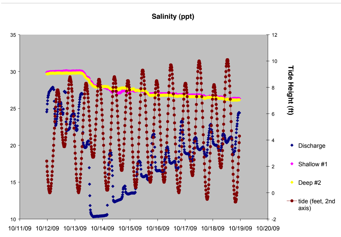
Figure 3.2-20: Pond A3W salinity values at 3 pond locations during 12 October – 18 October
