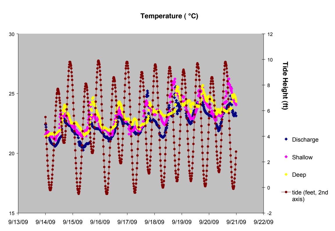
Figure 4.4-16: Pond A14 temperature values at 3 pond locations during 14 September – 20 September
