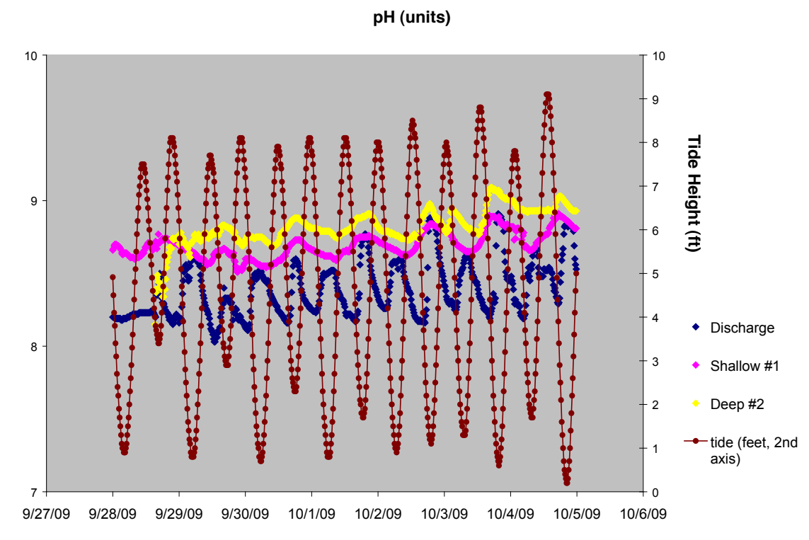
Figure 3.3-18: Pond A3W pH values at 3 pond locations during 28 September – 4 October
