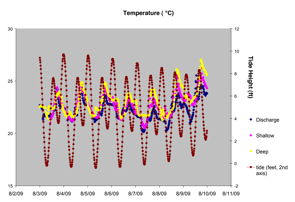
Figure 4.4-10: Pond A14 temperature values at 3 pond locations during 3 August – 9 August
