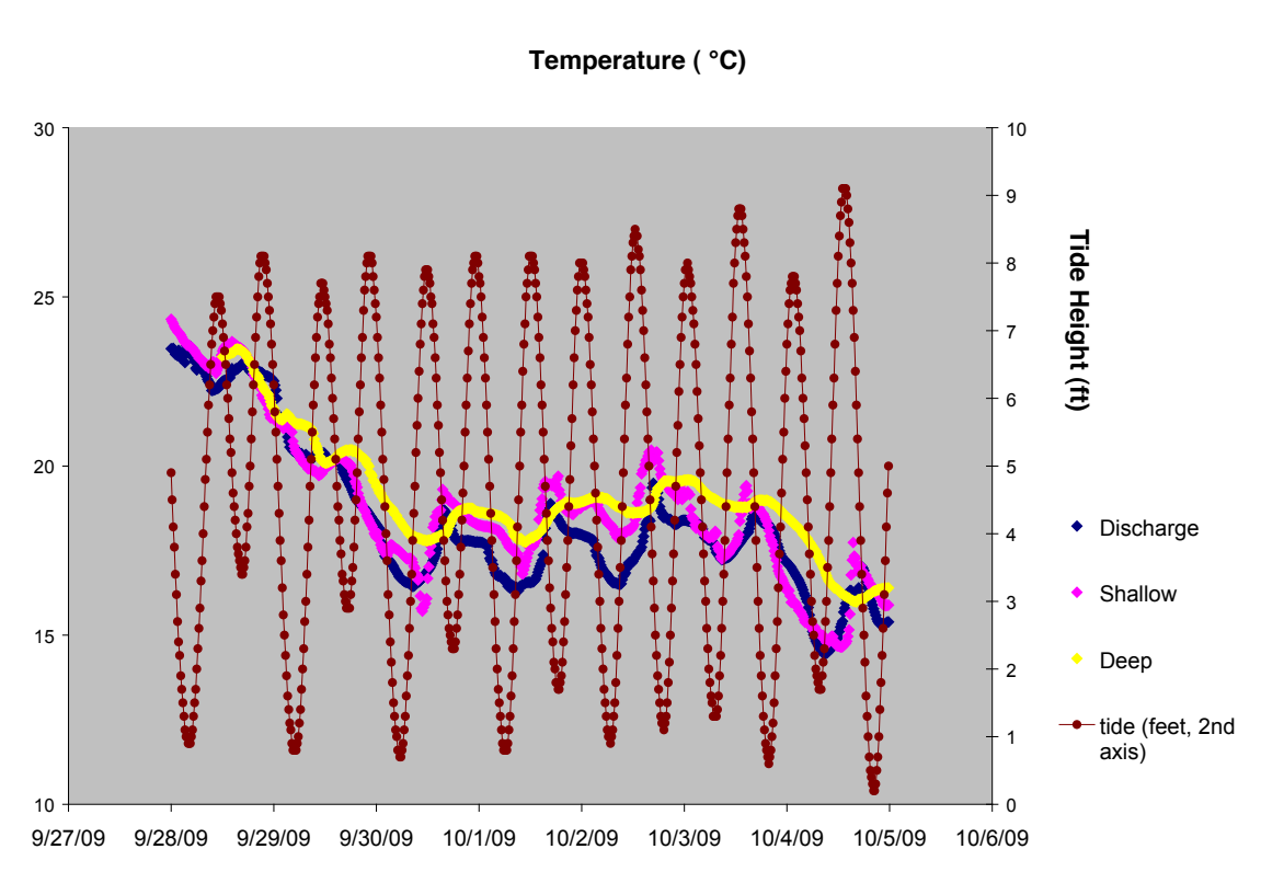
Figure 4.4-18: Pond A14 temperature values at 3 pond locations during 28 September – 4 October
