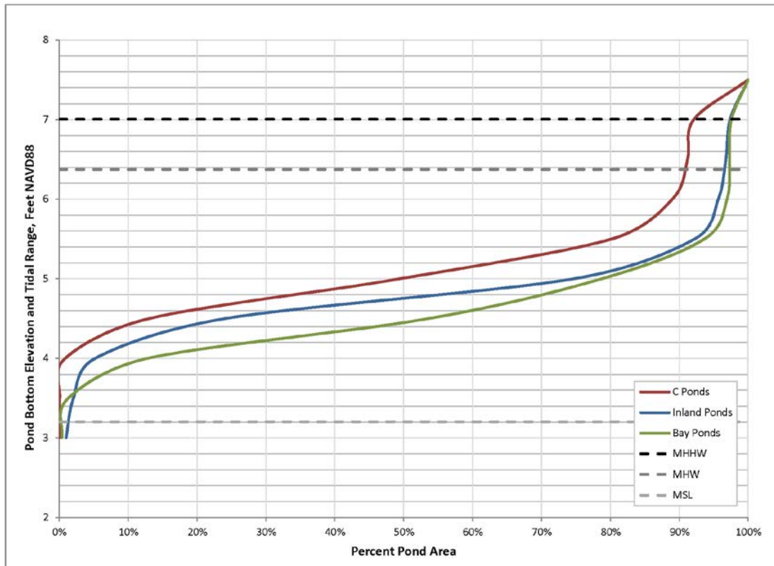
Figure 2.1. Average Pond Group Bottom Elevations
