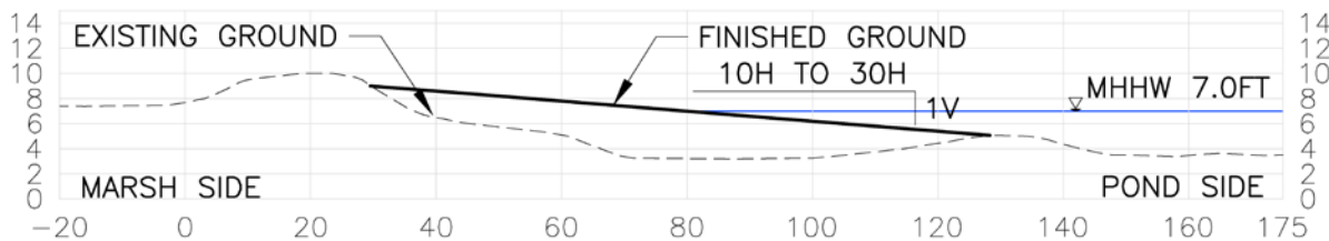
Figure 4.19. Proposed Habitat Transition Zone – Typical Section
