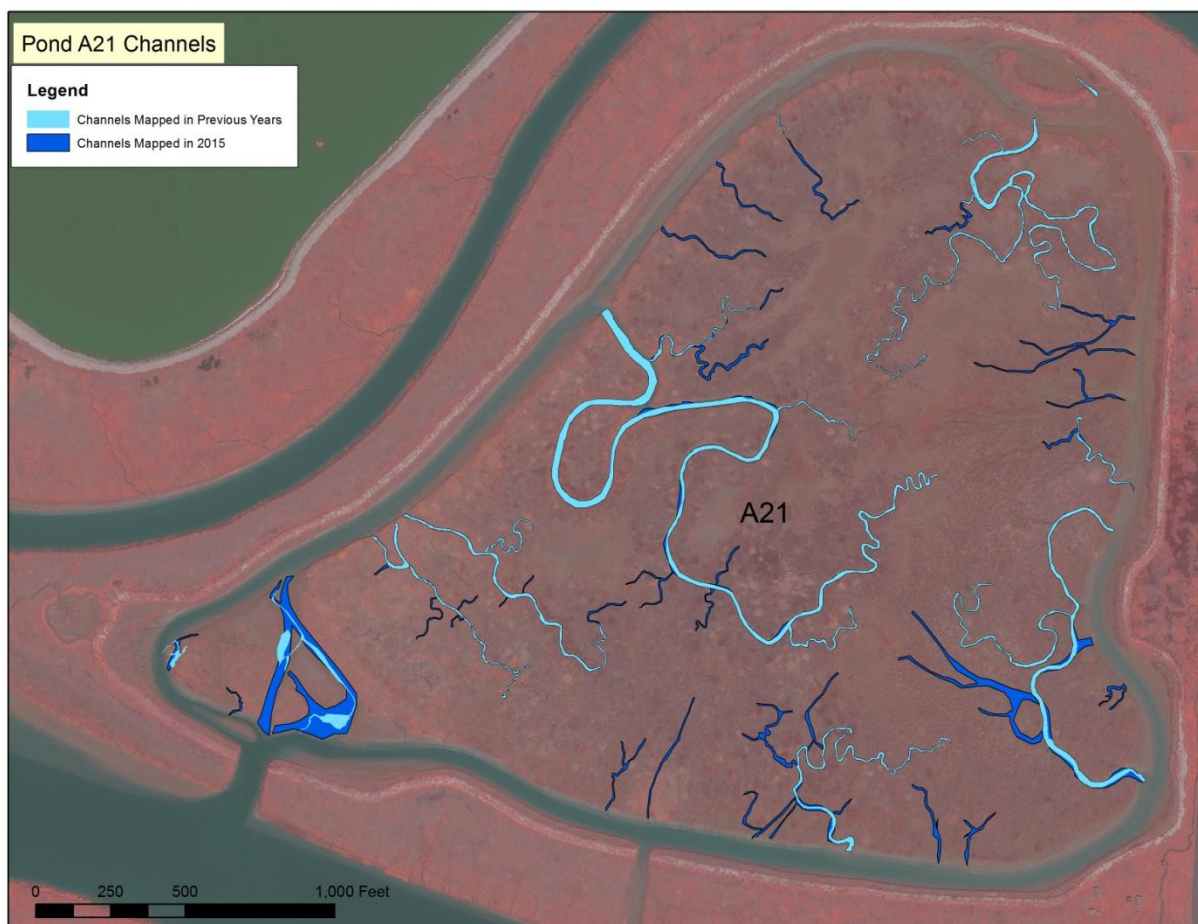
Figure 5. Channel Geometry in Pond A21, 2015 Compared to Previous Years
