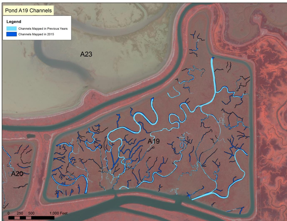
Figure 7. Channel Geometry in Pond A19, 2015 Compared to Previous Years
