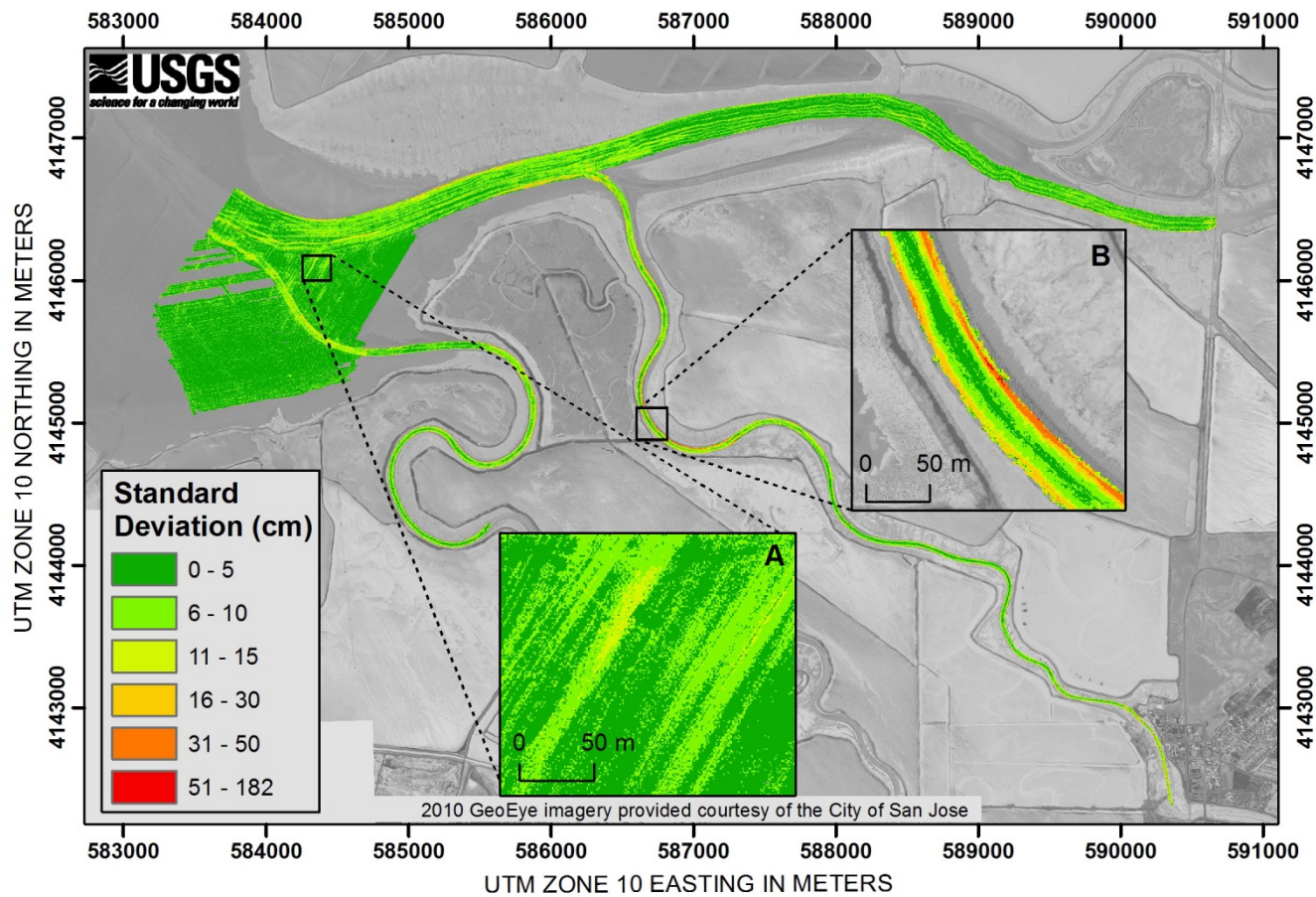
Figure 11. Plan-view map of bathymetric soundings standard deviation within each 1 \times 1 m cell, south San Francisco Bay, California.
