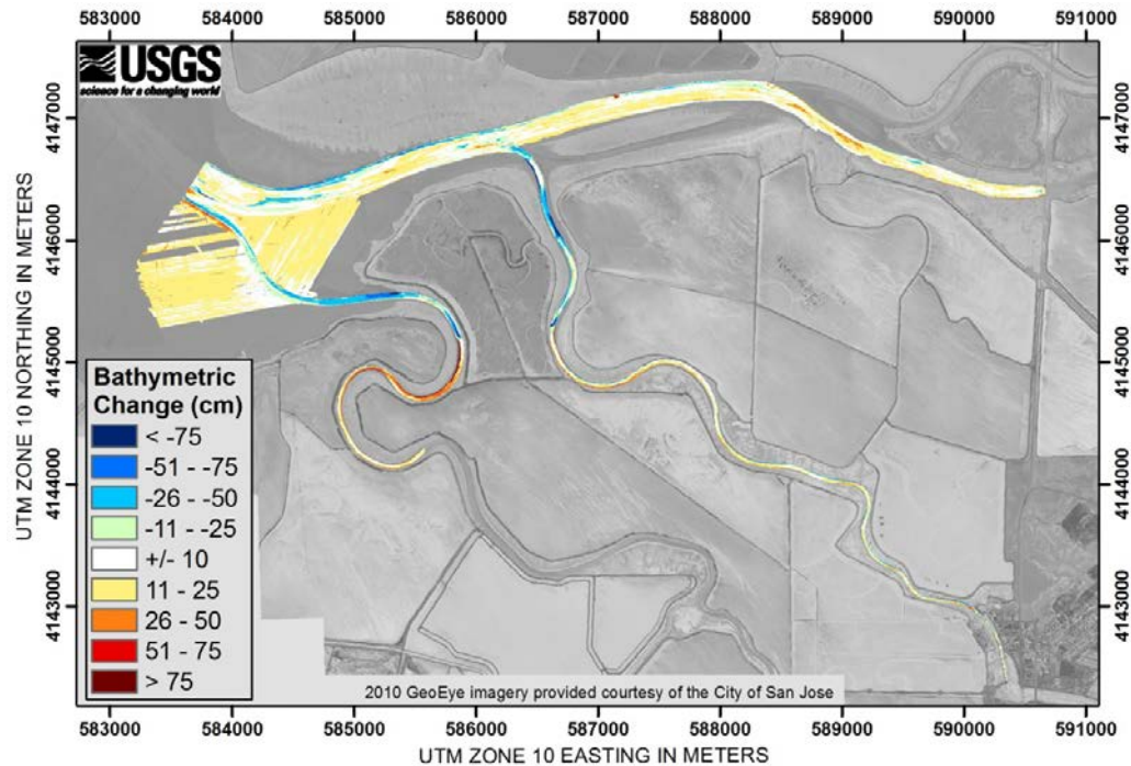
Figure 7. Bathymetric change from 2010 to October 2012.
